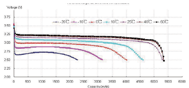
-20~60°C 1C Rate Discharge Curve
