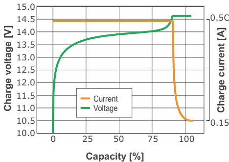
Charge Characteristics
